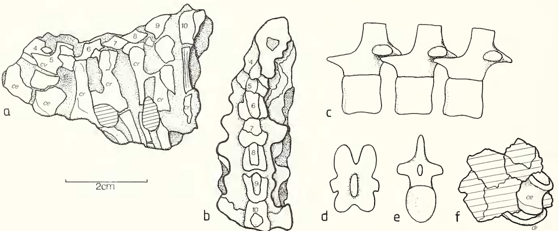
TEXT-FIG. 6. Vertebrae of juvenile Scaphonyx fischeri (MCZ 1664). a, b, cervical vertebrae 4-10, with associated cervical ribs, in left lateral (a) and dorsal (b) views. c, d, e, cervical vertebrae from the middle of the neck, restored in left lateral (c), dorsal (d), and anterior (e) views. f, Centrum of a dorsal vertebra and a dorsal rib in partial ventral view, embedded in matrix (diagonal shading).
